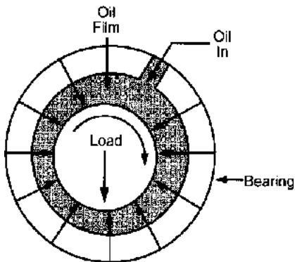
Fig. 7-23: Oil film in a hydrodynamic sleeve bearing.
