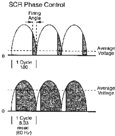
Fig. 8-34: The effect of the firing angle on the average voltage of a full-wave SCR control.
