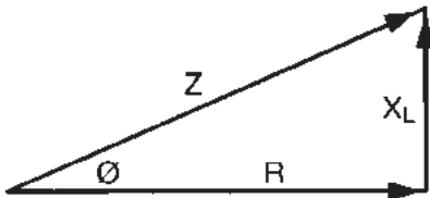
Fig. 1-38: Impedance diagram of an RL circuit.
