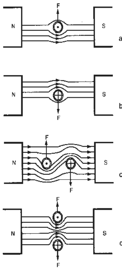
Figs. 3-1a, b, c, d: Upward and downward forces created by interaction of field and armature flux.
