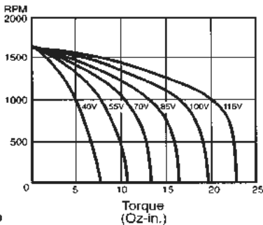
Fig. 8-22: a) Variable voltage transformer method in a PSC motor (top), and b) varying PSC motor speed by the variable transformer method (bottom).
