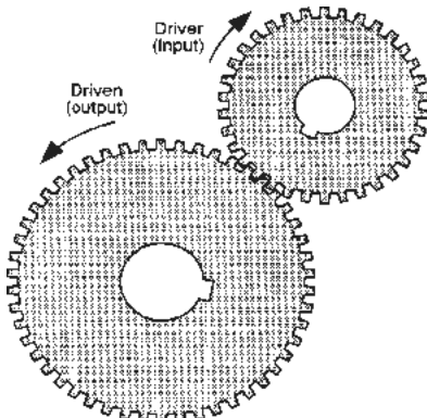
Fig. 6-1a: External-toothed spur gears.
