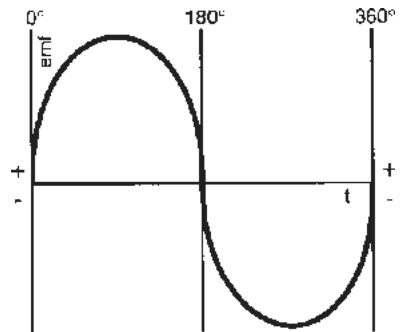
Fig. 1-24: Sine wave characteristic of AC current during one cycle ( 360^\circ ).
