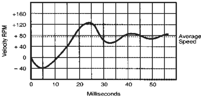
Fig. 4-1: Typical starting characteristics for a low speed AC synchronous motor.
