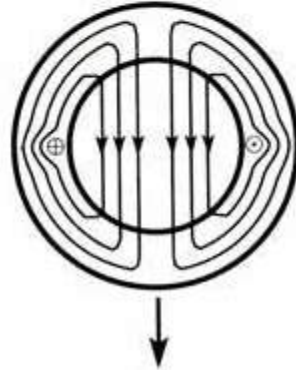
Fig. 2-4: Magnetic field set up when phase 1 is in negative cycle.
