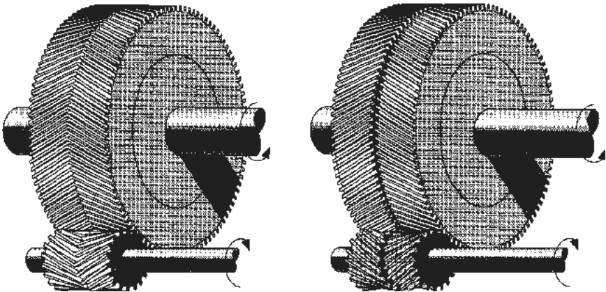
Fig. 6-4: Double helical and herringbone gears.
